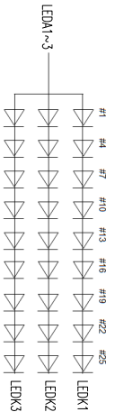
BACKLIGHT CIRCUIT DIAGRAM
