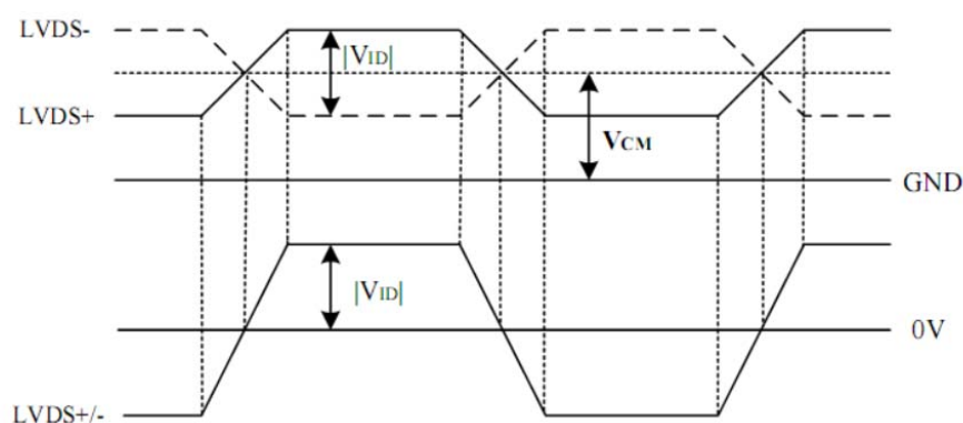
Figure 1 Voltage Definitions
