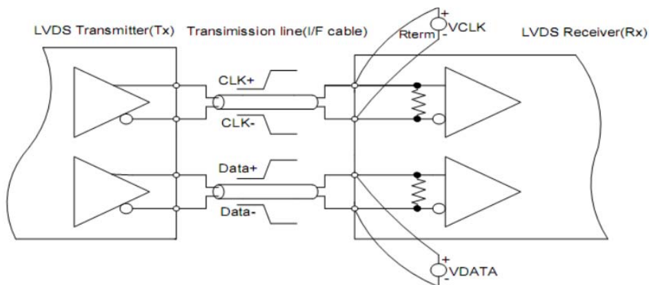
Figure 2 Measurement System
