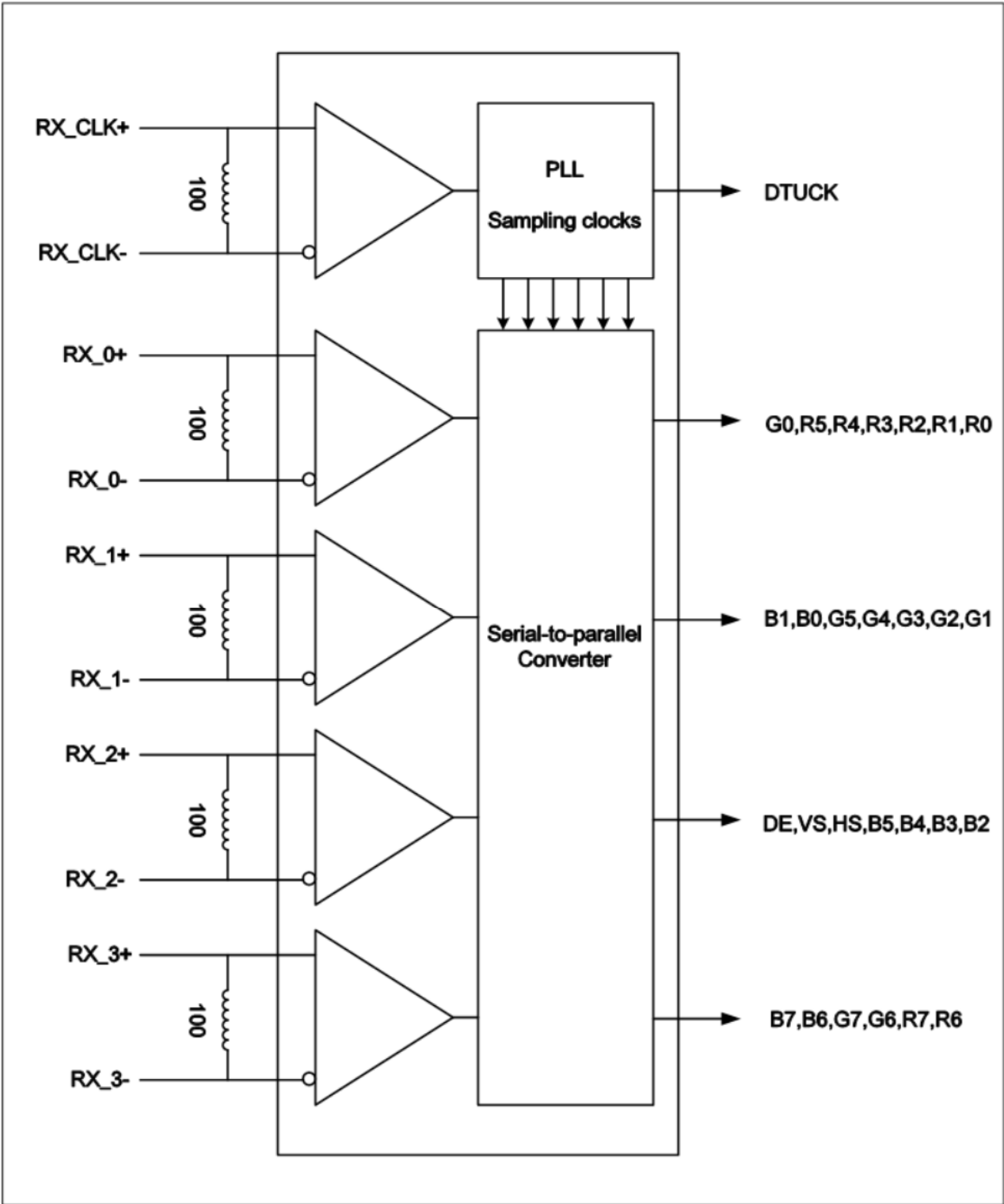
Figure 4 LVDS Receiver Internal Circuit
