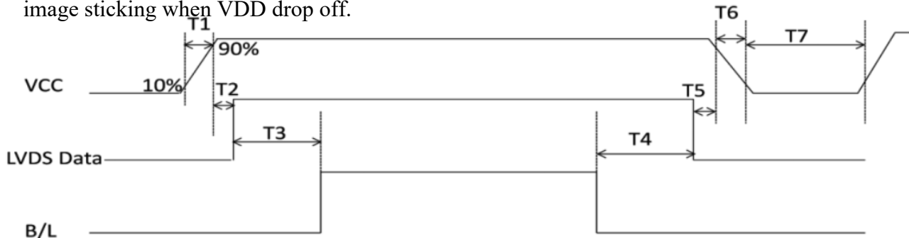
Figure 5 Power Sequence
