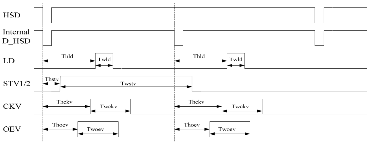
Gate output Timing Diagram (Dual Gate)
