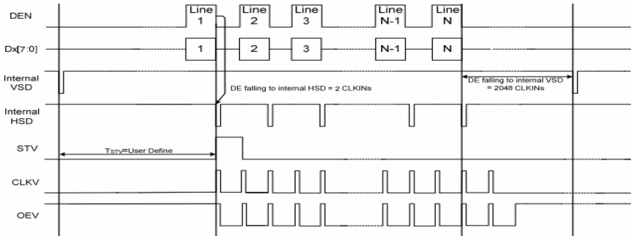
Gate output Timing Diagram (Dual Gate)
