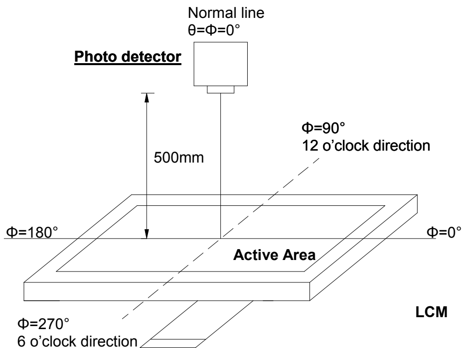
Fig. 4-2 Optical measurement system setup
