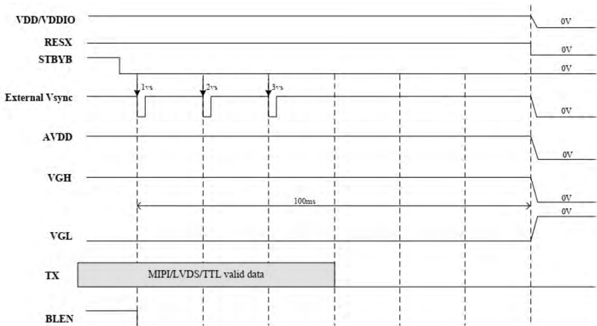
Figure: Power Off Timing Chart
