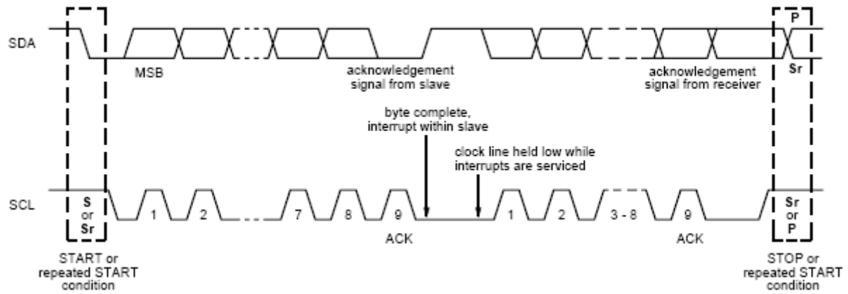
Figure 1-1 I2C Serial Data Transfer Format
