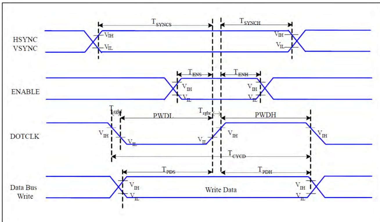
Figure 3. RGB interface timing characteristics
