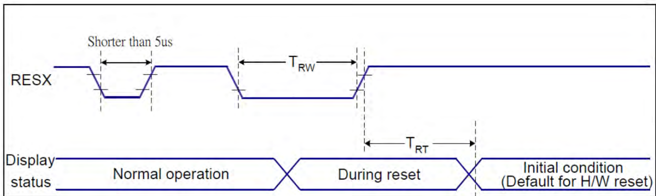
Figure 4. Reset timing
