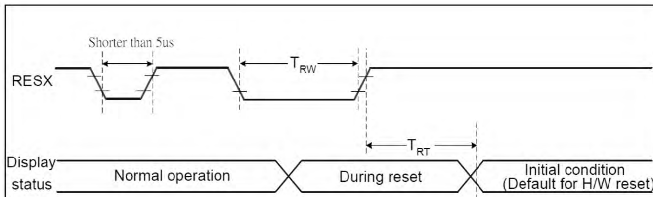
Figure 7. Reset Timing
