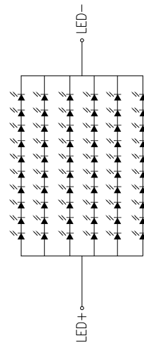
BACKLIGHT CIRCUIT DIAGRAM
