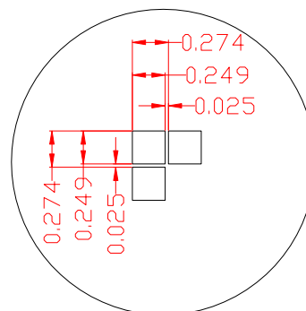
DOT DETAIL SCALE 10X
