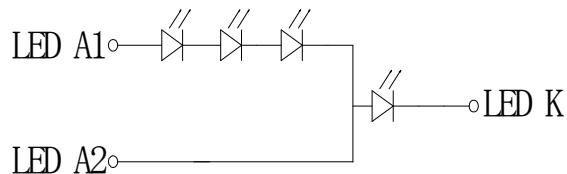
LED connection of backlight
