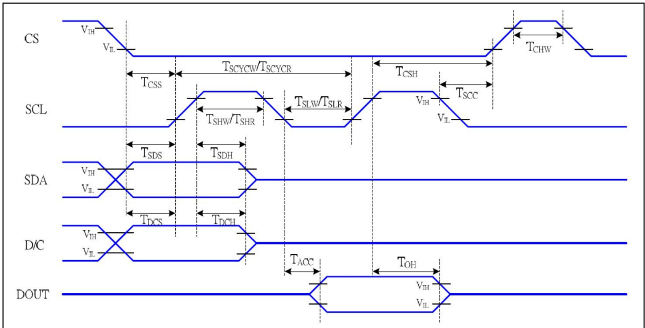
Figure 1 4-wire serial Interface Timing Characteristics
